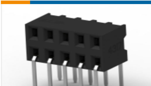
TE 产品编号1-2314916-0 10P, 2MM, B-B, REC, DRHZ, 2.1, 0.1AU, TB
