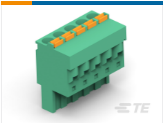
TE 产品编号 1986262-4 4 POS PLUG SPRING CONN, PITCH 5.08
