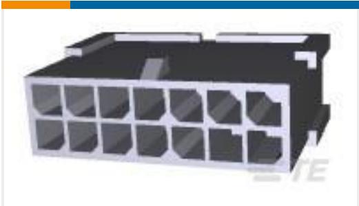
TE 产品编号1-794616-4 FREE HANG DBL ROW HSG 14 POS
