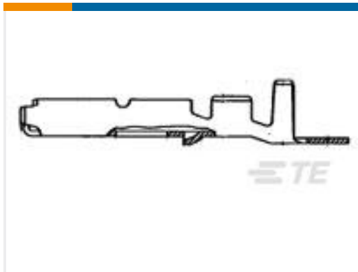
TE 产品编号172776-1 MIC MARK-2 REC CONTACT L.P.
