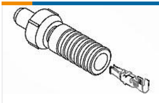
TE 产品编号863103-1 LGH CSL PLUG ASSY
