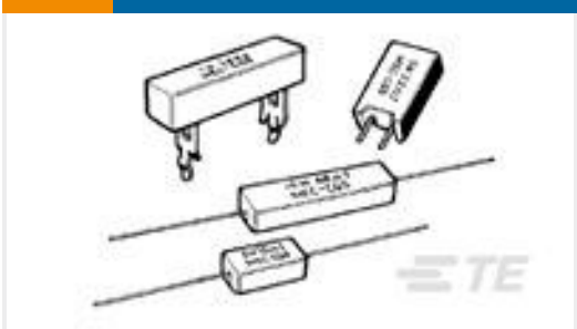
TE 产品编号1623783-7 SQM7 22K 5% (METAL FILM)
