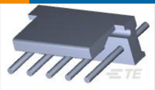
TE 产品编号3-644760-5 05P MTA156 HDR ASSY FL ST LF
