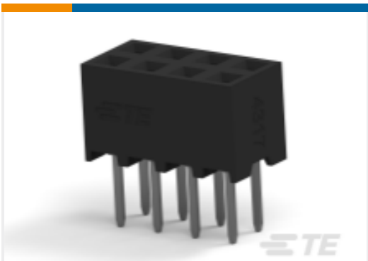
TE 产品编号2314820-8 8P,2MM,B-B,REC,DRVT,2,7,0.1AU,TB
