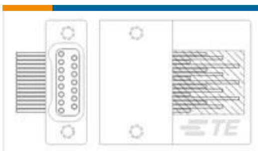
TE 产品编号5-1589487-4 STM065M6SN = THRU-HOLE
