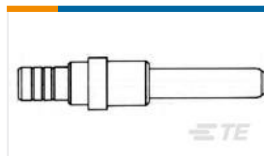
TE 产品编号 1738025-1 Pin Contact, Size 15
