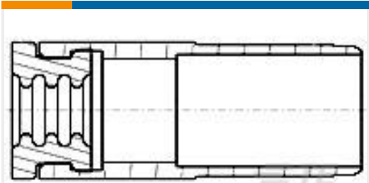
TE 产品编号1757824-8 AMPLIMITE,ASY,RCPT,STD,90,ZN,2, CONT
