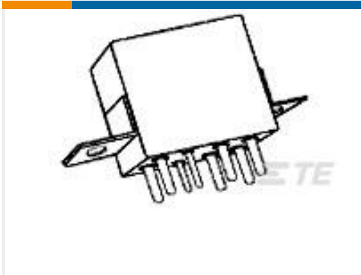
TE 产品编号5-1617758-1 FCB-205-0225M=M83536/2-025M
