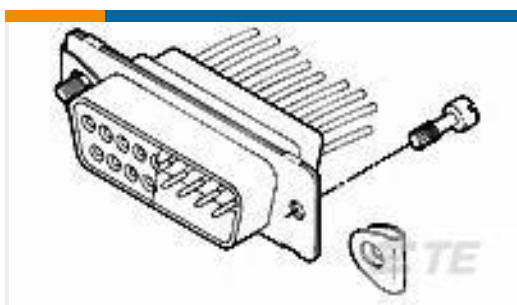
TE 产品编号 5205980-1 SCREW RETAINER KIT
