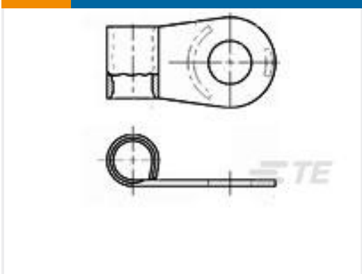
TE 产品编号321576 TERM,SOLIS, FLAG, R, 6, 1/4
