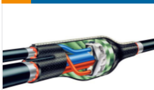
TE 产品编号543790-000 BMHM-1001-4C1-6878(S4)
