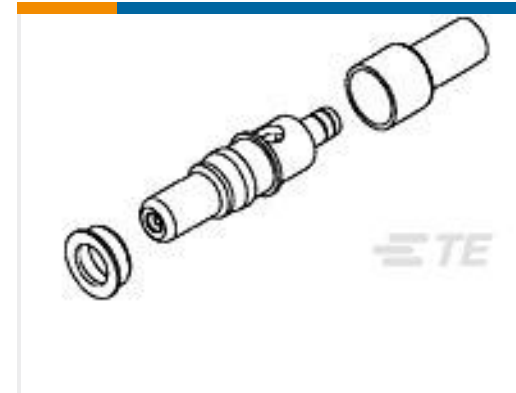
TE 产品编号221980-1 PIN,STRAIGHT,SIZE 8,50 OHM
