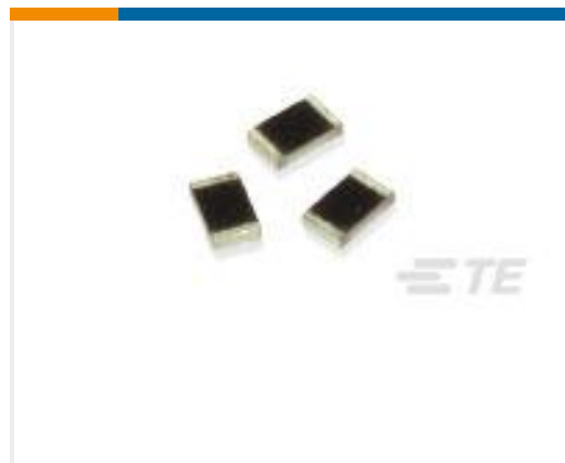
TE 产品编号1622818-3 RH73 2A 4M7 5% 250PPM
