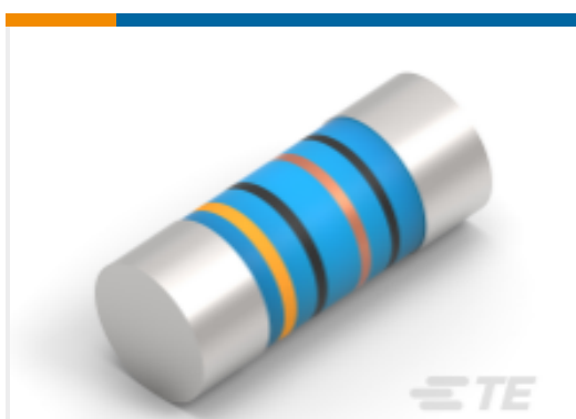
TE 产品编号5-2176314-3 MELF SMA_A 3K3 1% 50PPM 0102 0.3 W
