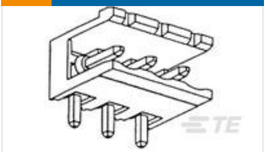
TE 产品编号282817-5 TERMI-BLOK HEADER,ASSY90 5P.
