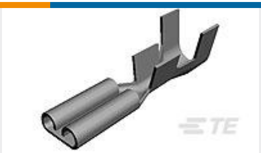
TE 产品编号170213-2 250 FASTON,REC.,18-14 AWG,TPBR
