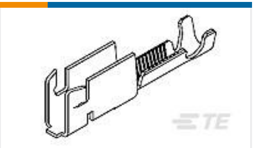
TE 产品编号1217671-1 CLSTR BLK RCPT AMVAR 1500-4200
