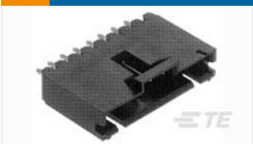
TE 产品编号103639-5 06 MTE HDR SRST LATCH .100CL
