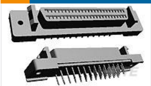
TE 产品编号749721-7 68 50SR VERT RCPT ASSY
