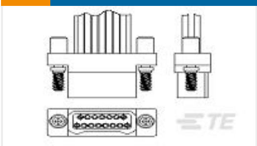
TE 产品编号8-1589474-1 STM051PC2DC036N = WDUALOBE
