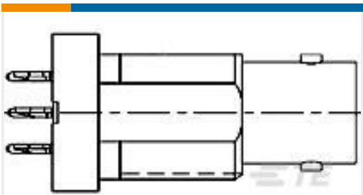
TE 产品编号5415456-1 JACK,PCB,PIN,BNC,75 OHM
