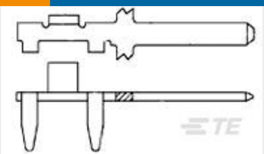
TE 产品编号1217183-1 FASTON,SPECIAL FLAG,TAB,TNBR
