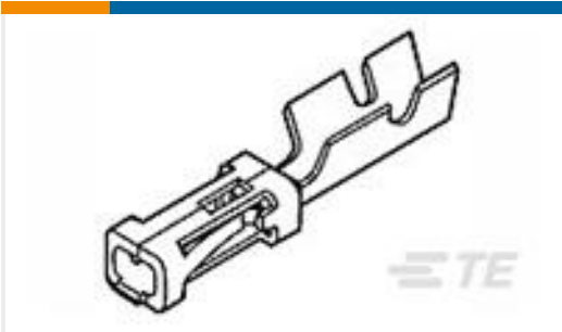
TE 产品编号2-160759-1 POSITIVE LOCK 250 REC 0.5-1.5MM2 NPPHBRZ
