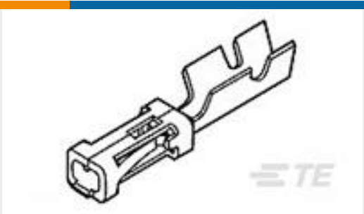
TE 产品编号1-794608-0 PIN CONT 20-24 TIN PLATE STRIP
