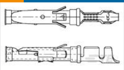
TE 产品编号163083-8 .062 DIA SOC.ASS.3+
