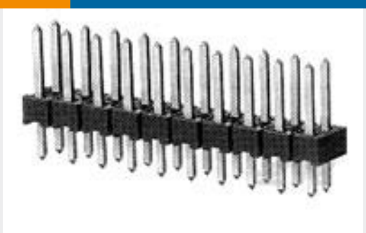
TE 产品编号102973-6 12 MODII HDR DRST B/A .100CL
