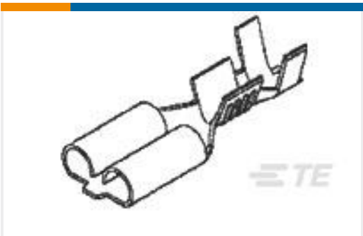
TE 产品编号170032-5 250 FASTON, REC., 20-14 AWG, TPBR
