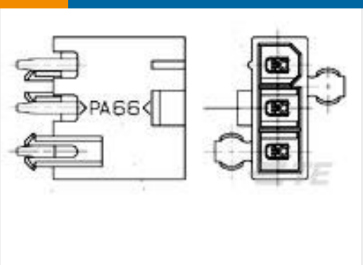
TE 产品编号2029113-3 3P VAL-U-LOK VRTHDR W/PGS GW
