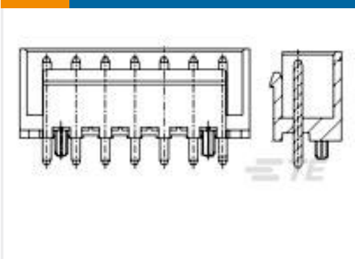
TE 产品编号1744357-3 3.96 EP SHROUDED HDR ASSY 3P W
