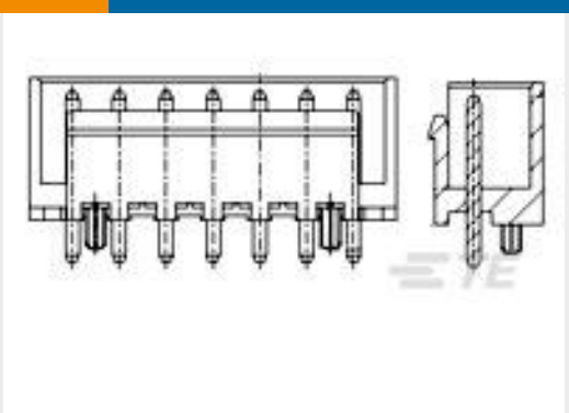
TE 产品编号1744357-5 3.96 EP SHROUDED HDR ASSY 2P W
