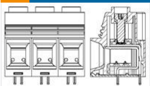
TE 产品编号1986242-4 Power Connector, 15.0mm, Green, 4 posn
