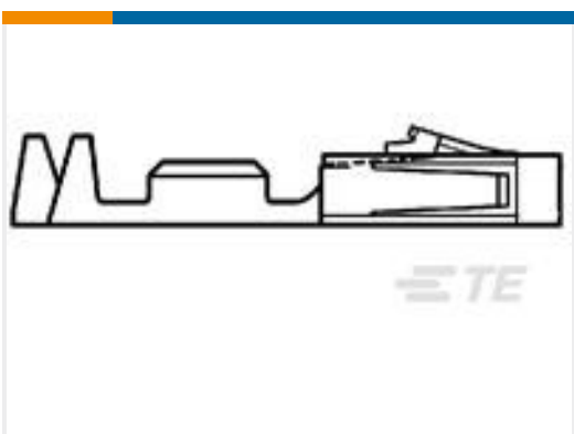
TE 产品编号104479-3 SHORT POINT CONT 15 DPLX STMPD
