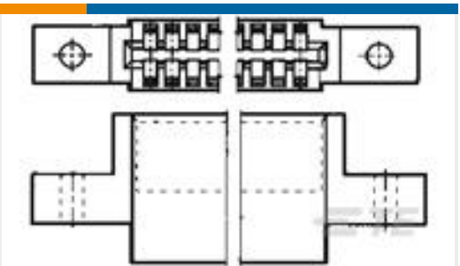
TE 产品编号1-583718-5 TW LEAF CRP HSG. 40-POS.
