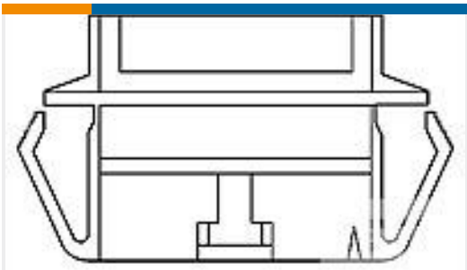
TE 产品编号103682-1 02 MTE PANEL MOUNT SR
