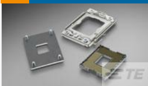
TE 产品编号1939738-1 ILM COVER ASSY, LGA1366
