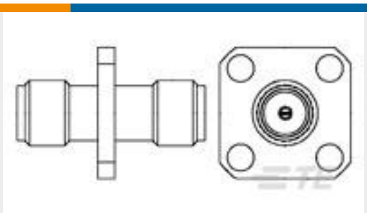
TE 产品编号1054988-1 SMA Jack-Jack Adapter 2084 8002 92
