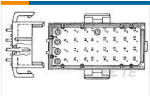
TE 产品编号1318699-1 MR HDR ASSY 3P COATING
