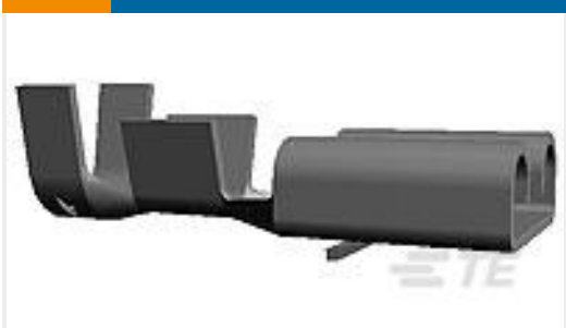
TE 产品编号160811-5 FF 250 REC 4-6MM2 BR SILVER PLATED
