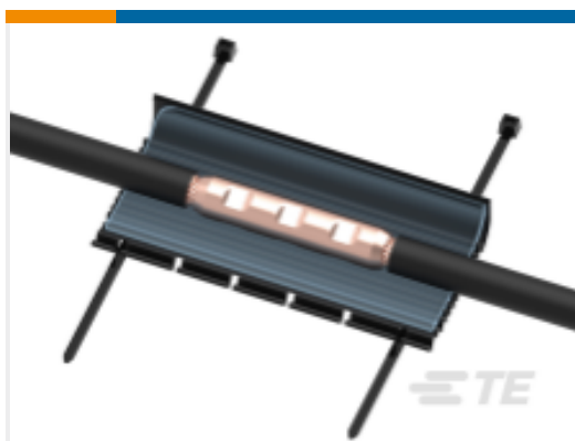
TE 产品编号C28893-000 GELWRAP-33/10-250(B6)-DE
