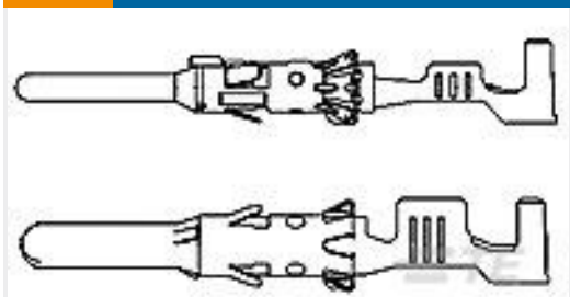
TE 产品编号1703013-8 DIA 1.5MM CONTACT PIN
