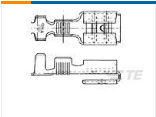
TE 产品编号160739-6 250 FASTON, PIGGYBACK REC., 18-14 AWG, PNST
