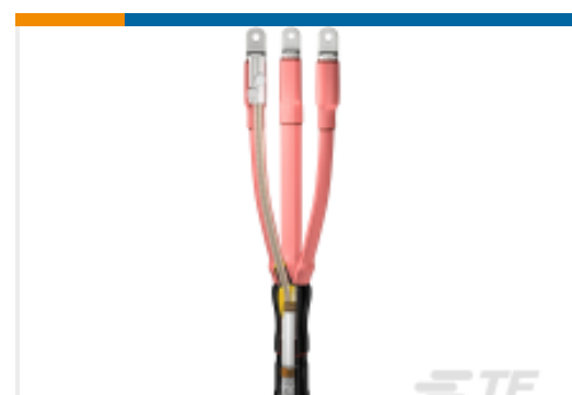
TE 产品编号C47372-064 GUST-12/25-50/800
