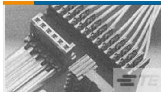
TE 产品编号144273-8 PLUG HE13 IDC 90 8 P AWG 24
