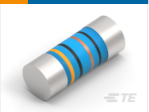
TE 产品编号2-2176314-0 MELF SMA_A 3K9 0.1% 15PPM 0102 0.3W
