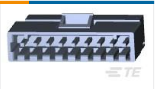
TE 产品编号3-647476-9 09P MTA156 PSTD CONN 18AWG LF
