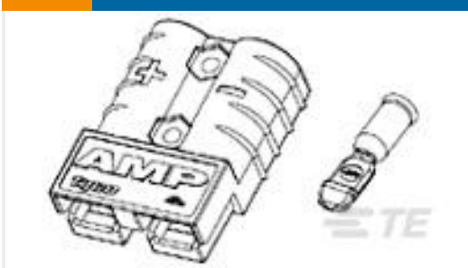
TE 产品编号647892-8 SRS 50 CONN KIT,YELLOW,6 AWG
