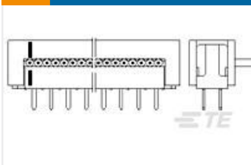
TE 产品编号6-216791-0 AMP LATCH D/P ASSY
