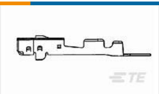
TE 产品编号179967-2 070 REC CONTACT "S" FORM
