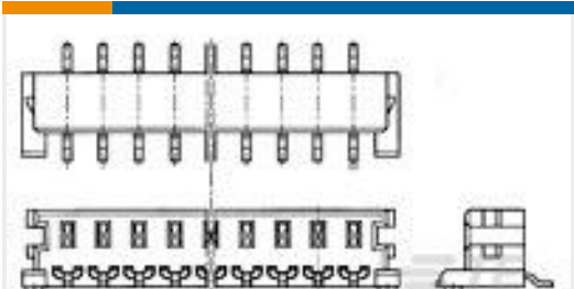
TE 产品编号1318182-2 DYNAMIC D3500 DUMMY HSG
