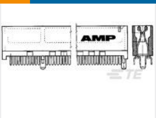
TE 产品编号1-5650090-2 STANDARD EDGE .050 SERIES 30 DUAL ASSY
