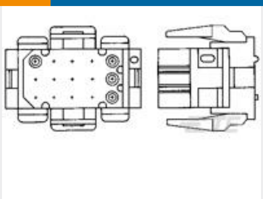
TE 产品编号1-640523-0 15P MR II PLUG HSG V0 RED
