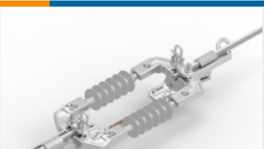
TE 产品编号1710725-4 15kILD-KR9C-T336.4-397.5
