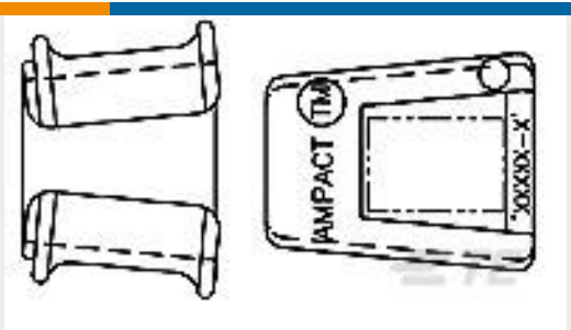
TE 产品编号602001 AMPACT Tap 336.4-1/0
